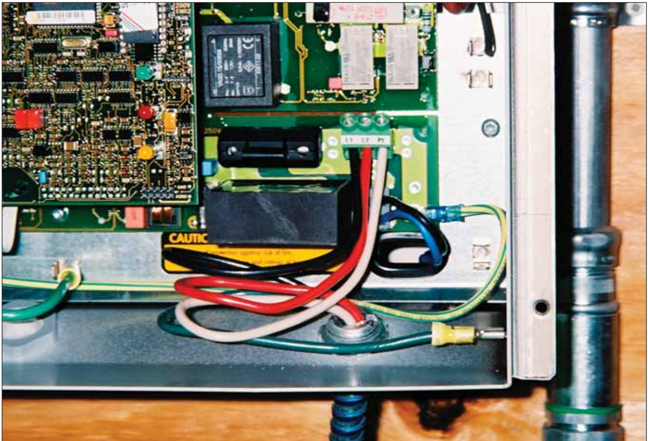
Photo 1. Improperly wired 240-volt inverter; neutral wired to PE terminal
