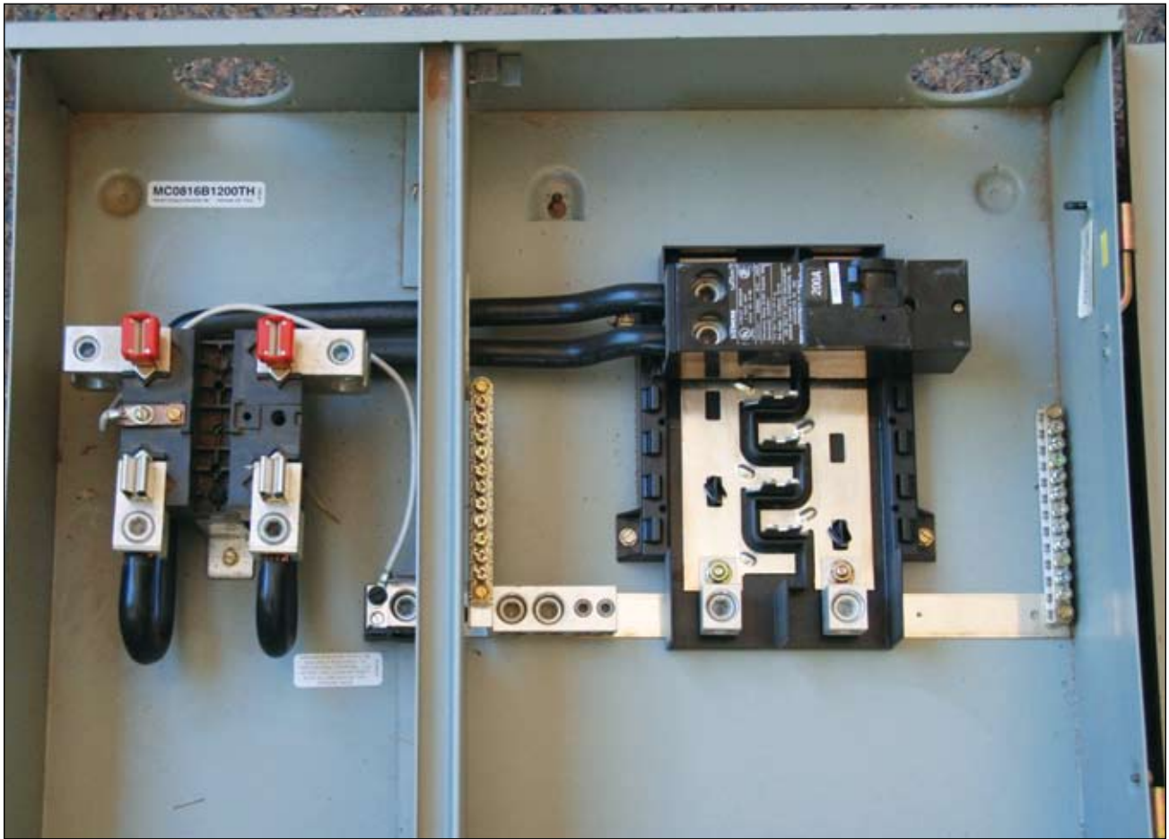
Photo 2. Much space but tap would violate the listing on the device
