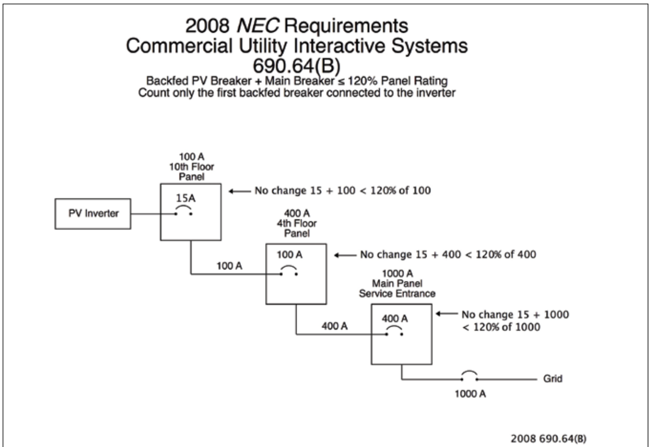
Figure 2. Section 690.64(B)(2) requirements in the 2008 NEC
