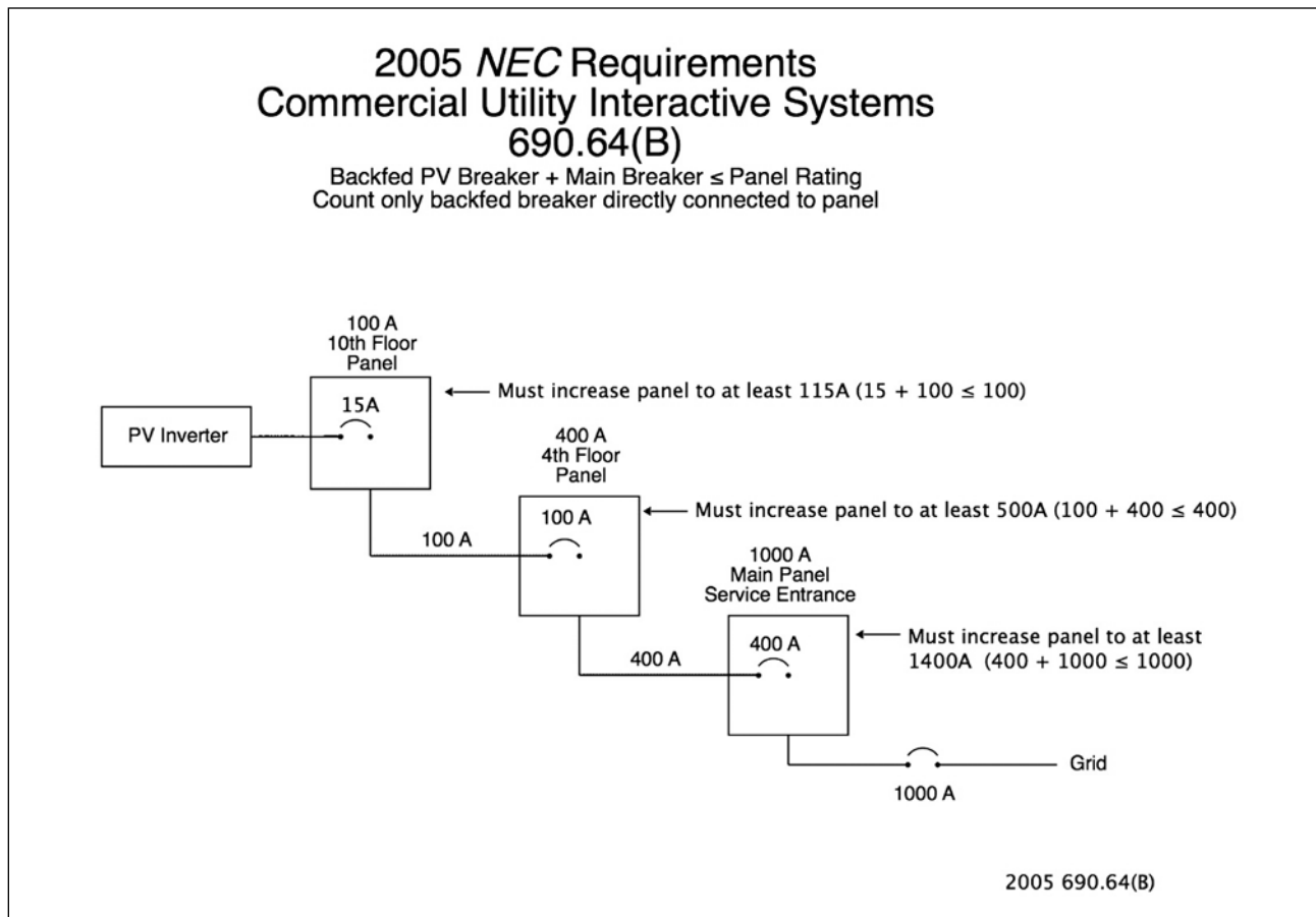
Figure 1. Section 690.64(B)(2) requirements in the 2005 NEC
