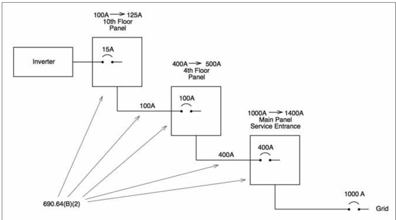
Figure 6. Multiple feeder panel connection diagram
