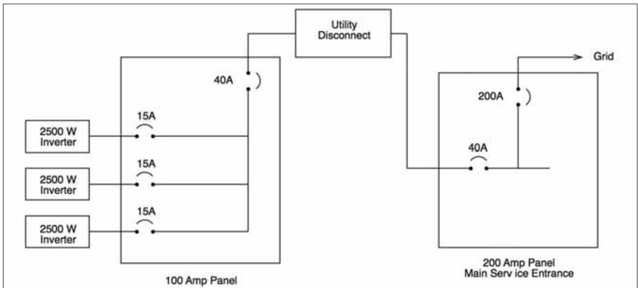
Figure 7. Three 2500-watt inverters on a 200-amp residential panel
