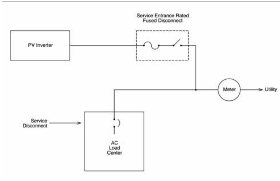
Figure 2. Supply-side interconnection diagram
