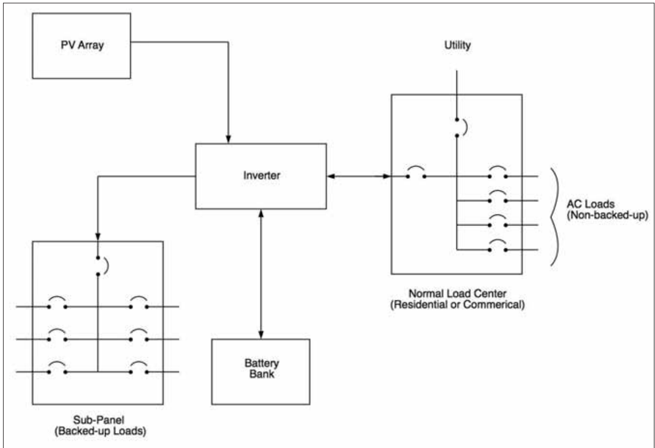
Figure 8. Utility-interactive PV system with battery backup
