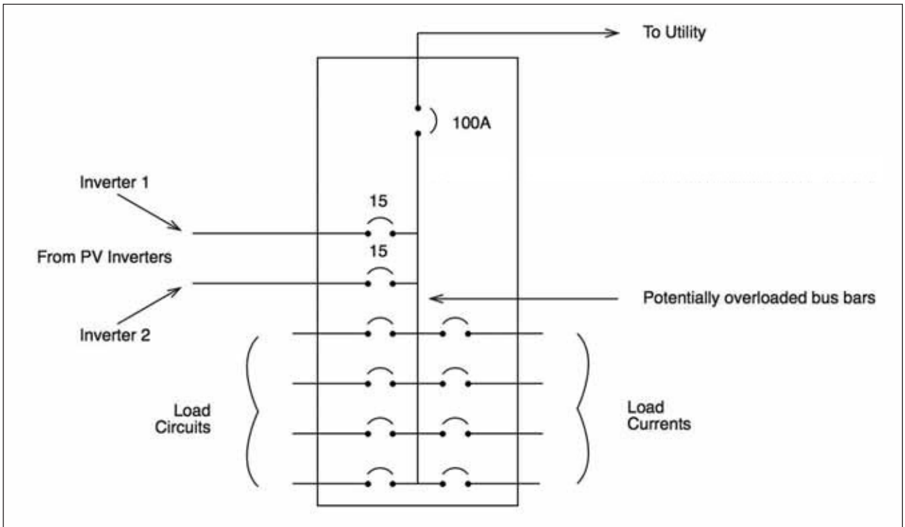
Figure 4. Load-side interconnection diagram
